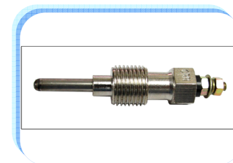
Glow Plug TL2300,2500,2700 Long: 74.40mm, Thickness 16mm CODE: 9-99-110-01
